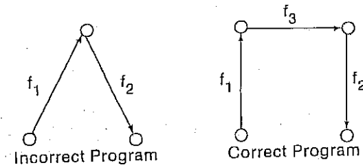
FIG. 4. Missing computational fault. (From Howden, copyright © 1985, IEEE).
