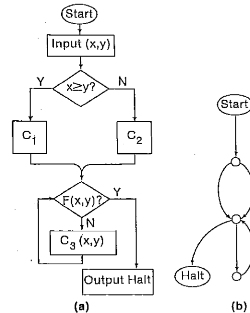
FIG. 2. Flow chart (a) and corresponding control flow graph (b).
