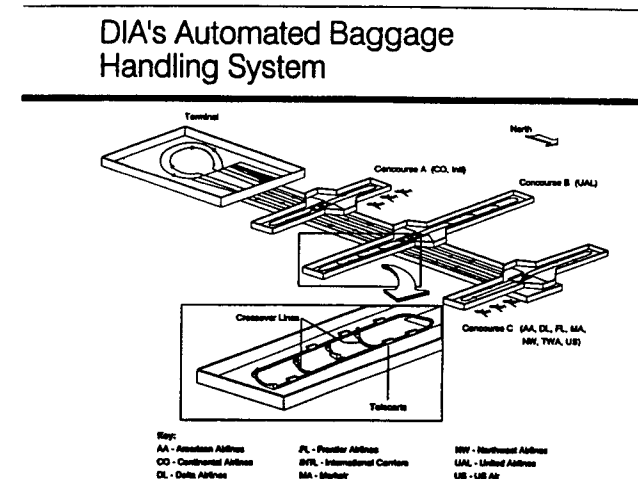
Figure 2. DIA's Automated Baggage Handling System [8]
